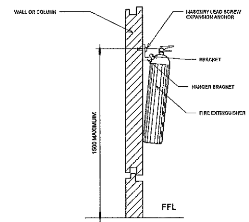
4 PORTABLE FIRE EXTINGUISHER DETAIL
